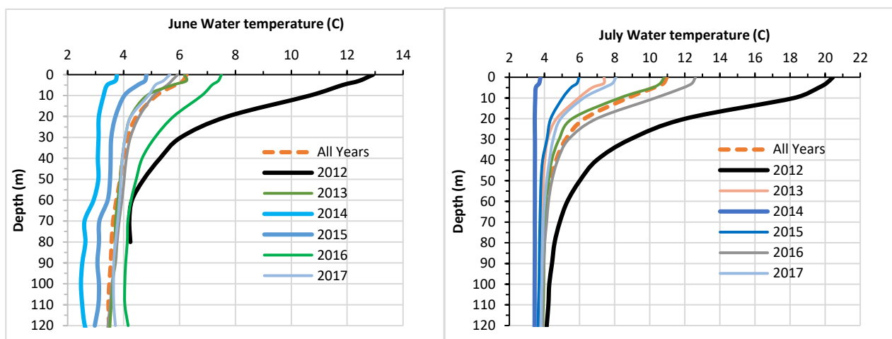
Figure 2. a) Average nearshore water temperature profiles collected in June. B) Average offshore water temperatures collected in July. All years is the average of temperatures collected from 1991-2017.
