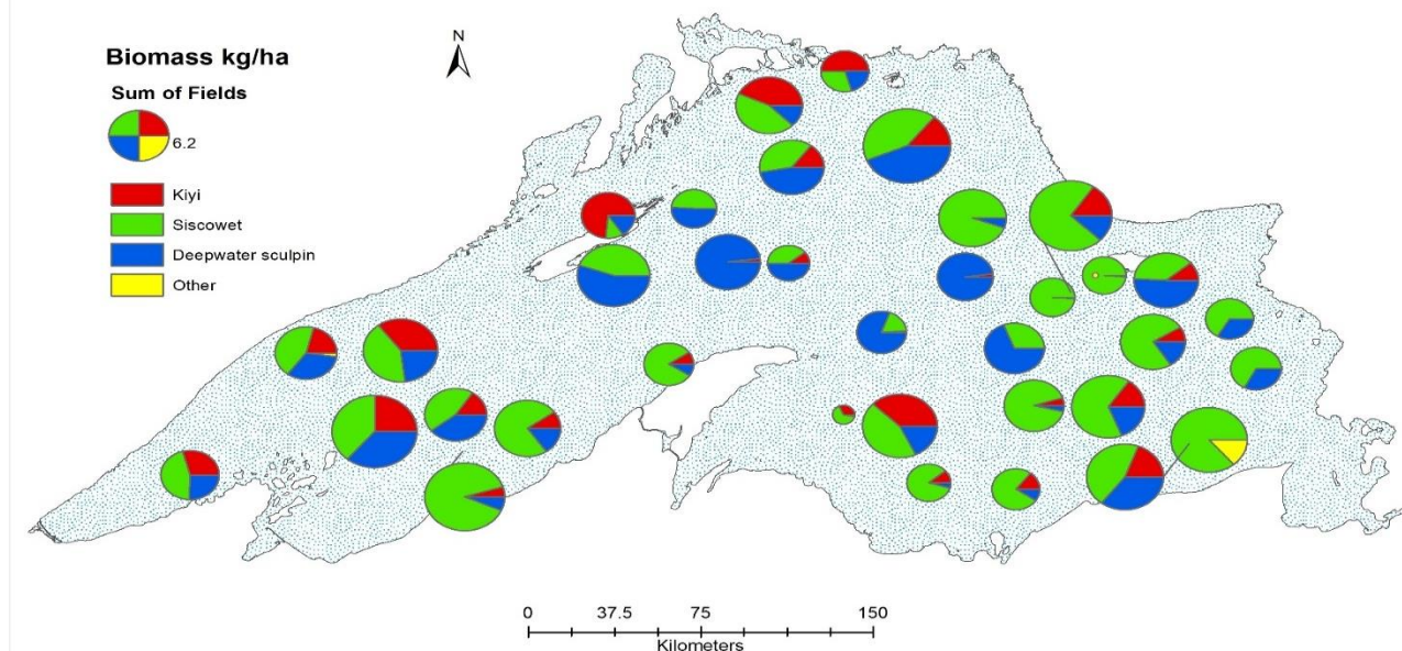
Figure 6. Mean lakewide biomass estimates for Kiyi, siscowet Lake Trout, Deepwater Sculpin, and other species estimated from offshore bottom trawls in 2017. Pie diameter is proportional to the biomass collected at that site, which ranged from 0.9-13 kg/ha. The pie in the legend is scaled to 6.2 kg/ha with the size of the pies on the map scaled accordingly to that reference.
