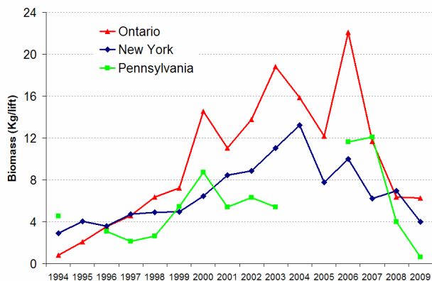
FIGURE 3.5 Average burbot biomass (kg/lift) from summer coldwater gill net assessment by jurisdiction, 1994-2009.
