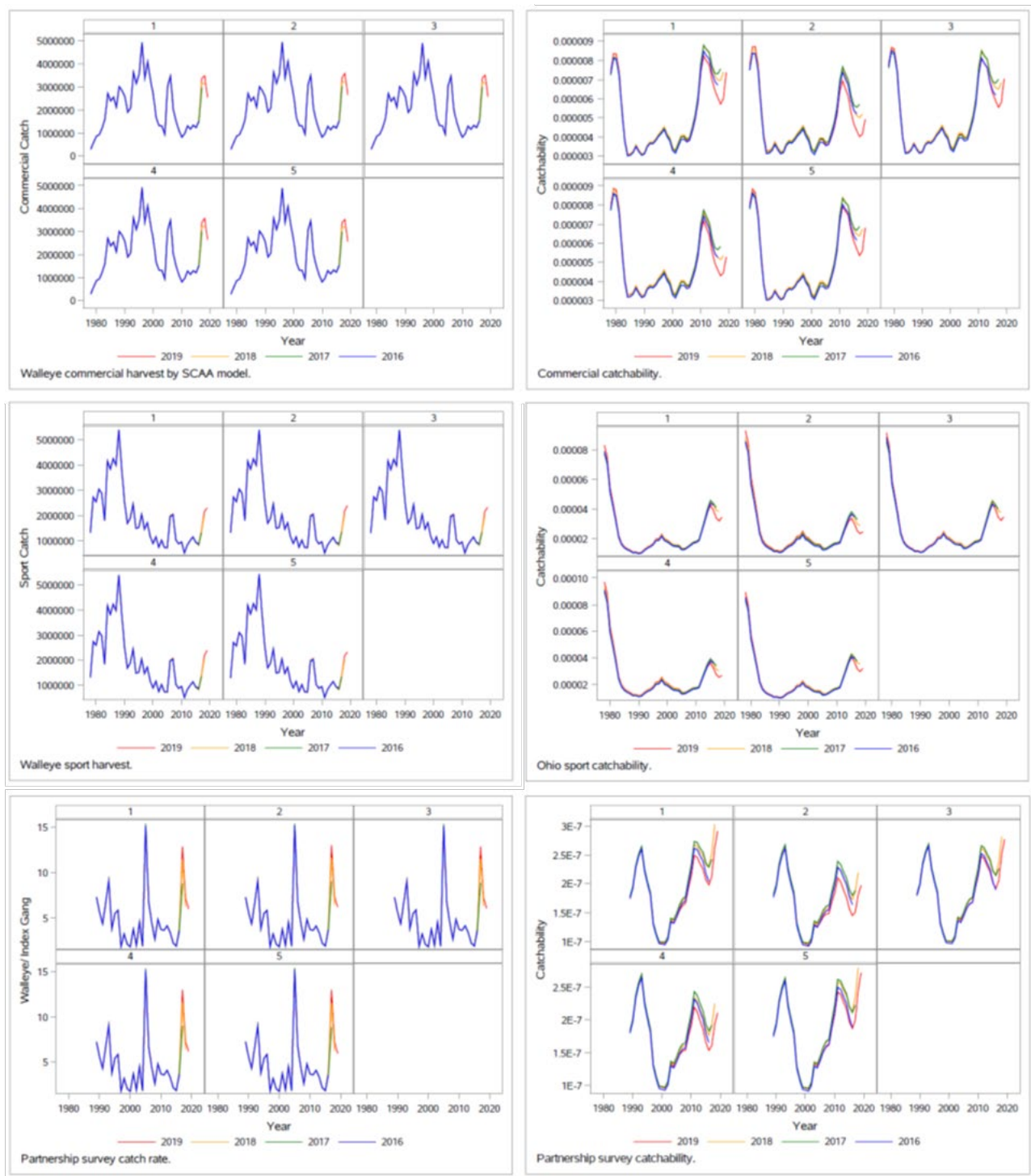
Figure A2: (continued): SCAA Model configuration retrospective pattern (Mohn's p ) by model output metric for 2019-2016, (see table A1 for model details).
