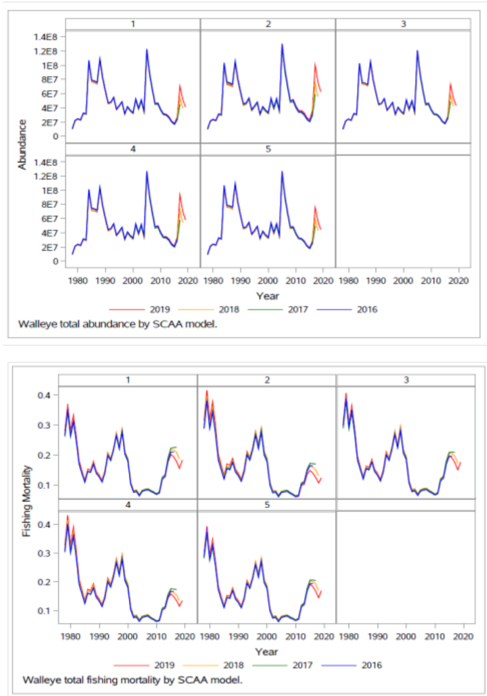
Figure A2: SCAA Model configuration retrospective pattern (Mohn's \rho ) by model output metric for 2019-2016, (see table A1 for model details).
